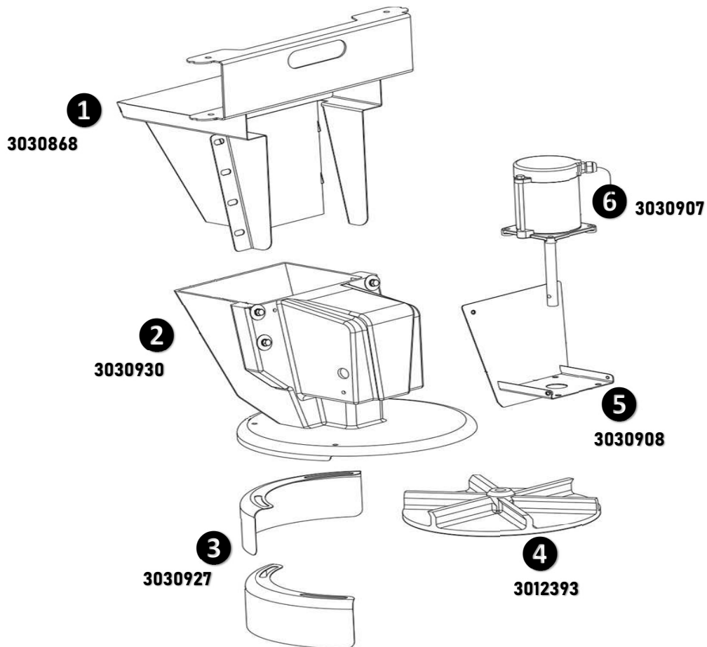
① Upper chute weldment 3030868
