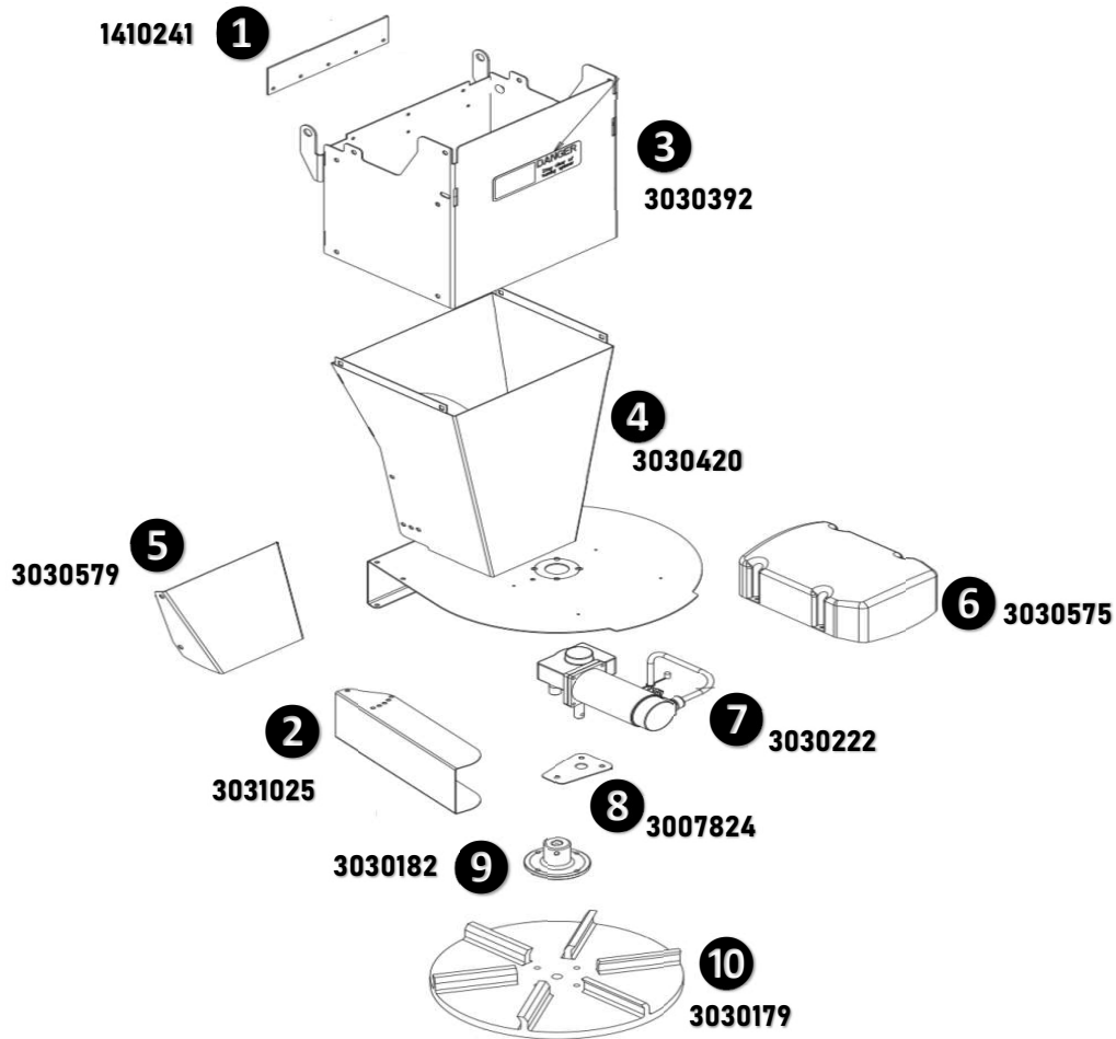
① Wipper belt hopper 1410241
