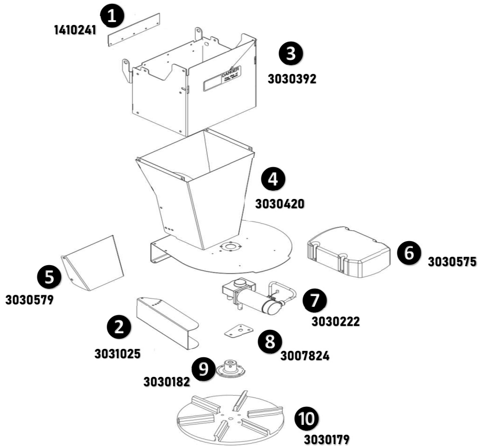
① Wipper belt hopper 1410241
