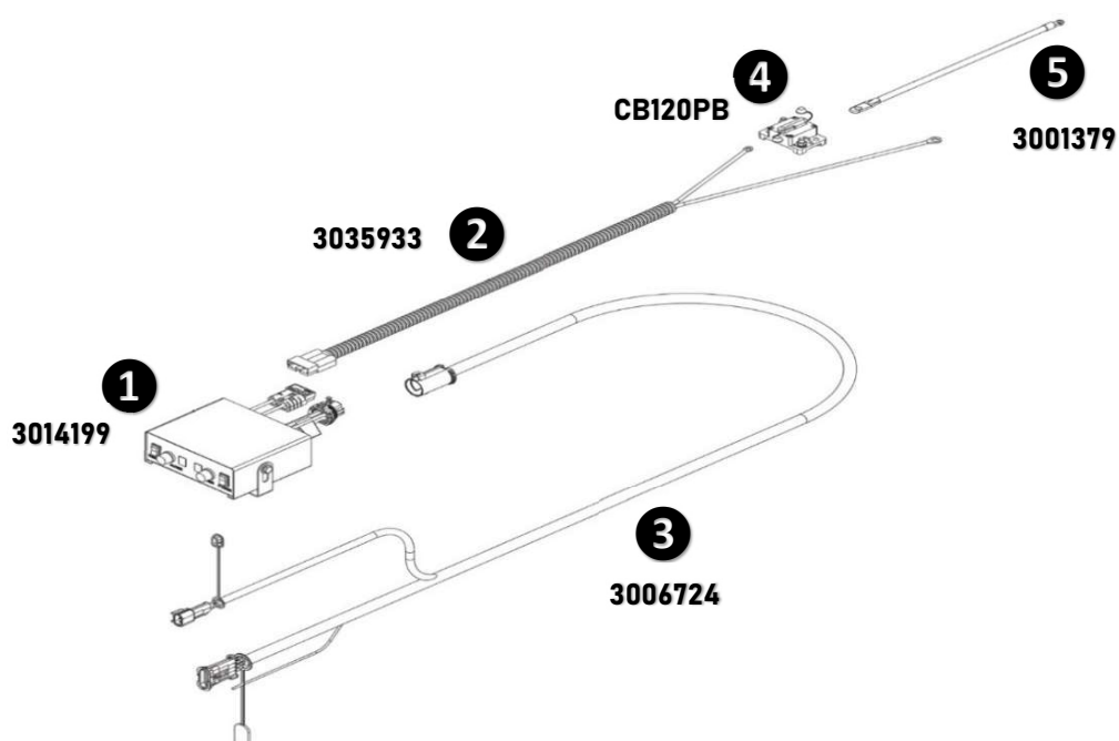
② Wire harness, power 3035933
